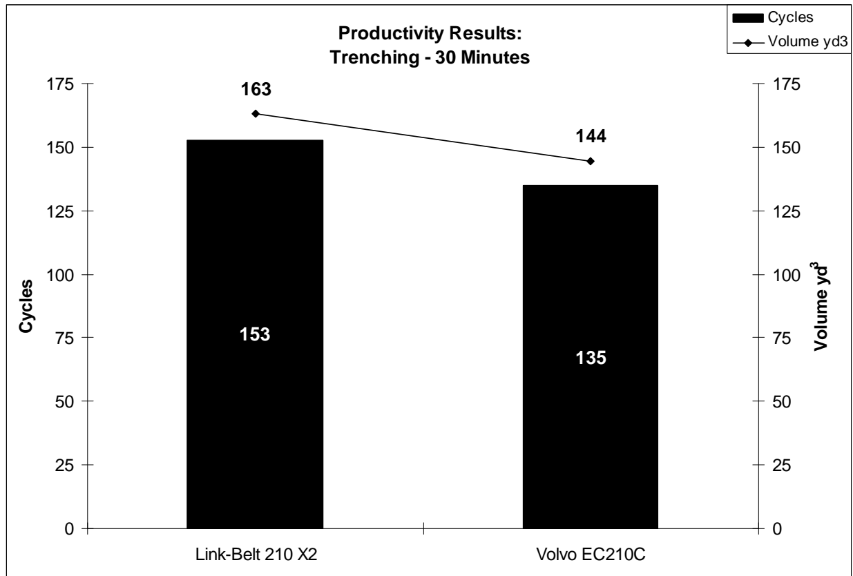
153 cycles were counted for the Link-Belt 210 X2 vs. 135 cycles for the Volvo EC210C over the 30 minute test, resulting in average cycle times of 11.8 seconds for the Link-Belt and 13.4 seconds for the Volvo. Total estimated volume of dirt moved was calculated by multiplying the number of cycles counted by a standard, heaped 1.07 yd 3 bucket.
